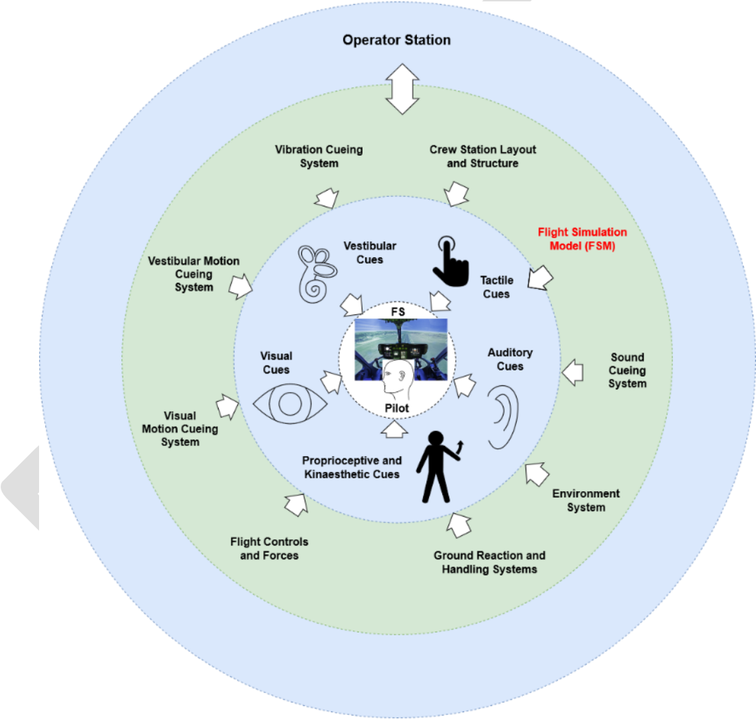
1919 1920 Figure 6-2: Schematic of FS Features
