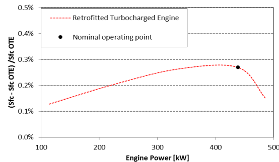
Figure 13: Sfc change for entire T/C retrofit.
