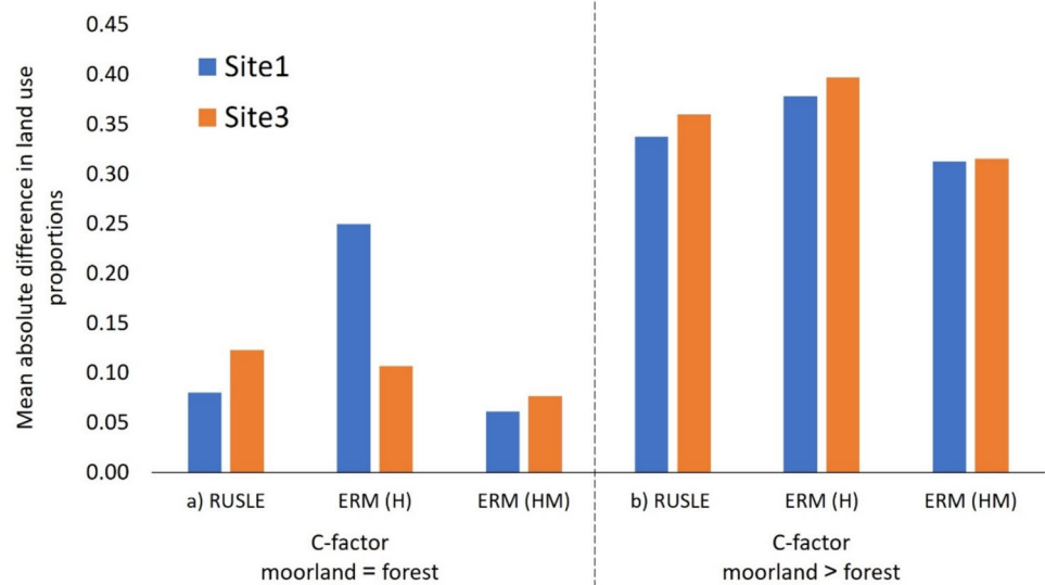
Fig. 5 For Sites 1 and 3 the mean difference between land use proportions estimated by the SF benchmark and a CLM RUSLE, CLM (H) and CLM ERM(HM) with the C-factor for moorland = forest, b CLM RUSLE, CLM (H) and CLM ERM(HM) with the C-factor for moorland > forest
