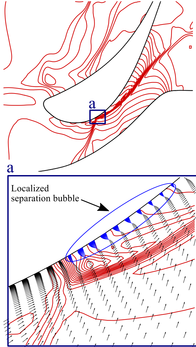
Figure 8: Shock wave interaction with the nozzle suction side boundary layer causing a localized separation zone. This flow behaviour is observed between time instances B and C of Fig.7. The isobar lines are shown in red, the velocity vectors in black, and the separation bubble velocity vectors in blue.
