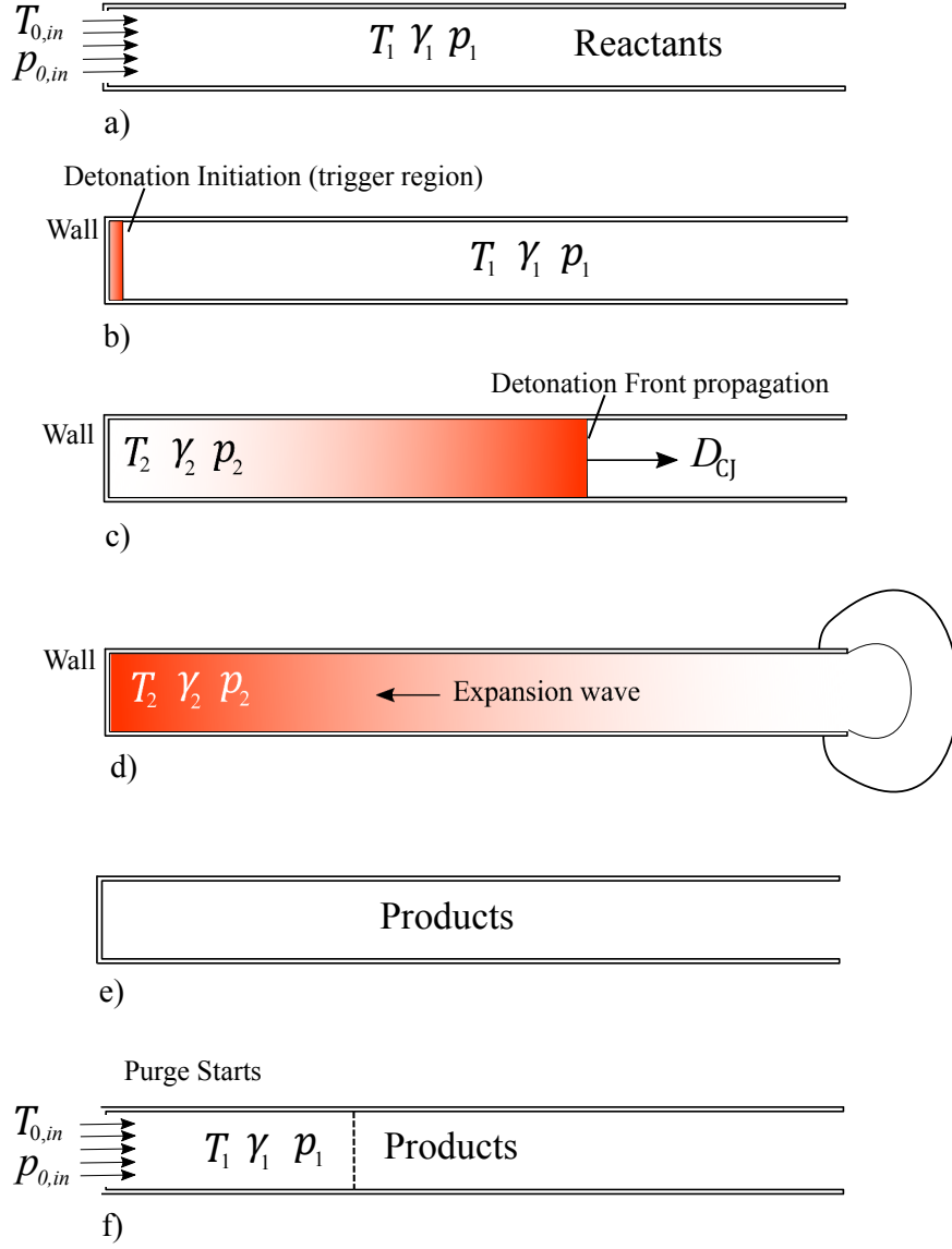
Figure 4: Different phases occurring in a PDC cycle [3]: a) filling ends; b-e) detonation initiation, propagation and blowdown; f) purge starts.
