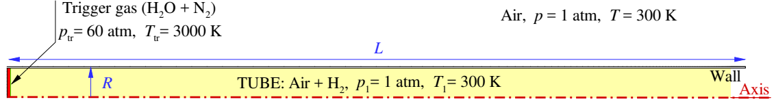
Figure 1: Partial view of the numerical domain used for the PDC-tube simulations, and initial conditions prior to detonation, R = 0.02 m, L = 0.5 m.
