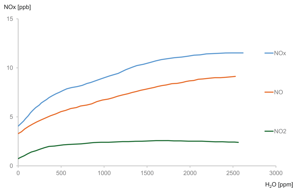
FIGURE 8 | Nitrogen oxides (NO x ) evolution from 5 g nitrocellulose (NC) sample (12.6%) heated at 60°C with a carrier gas flow rate of 40 mL/min.
