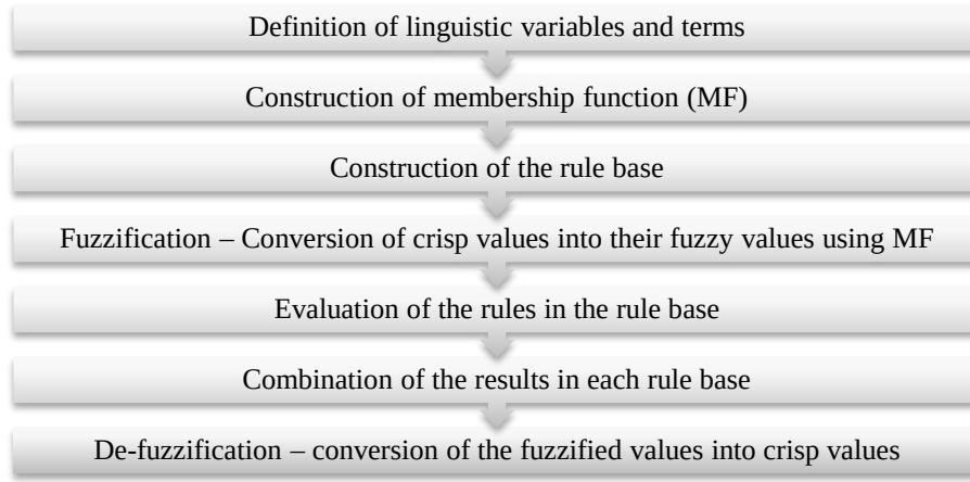
Figure 5. Main steps for a fuzzy logic algorithm.
