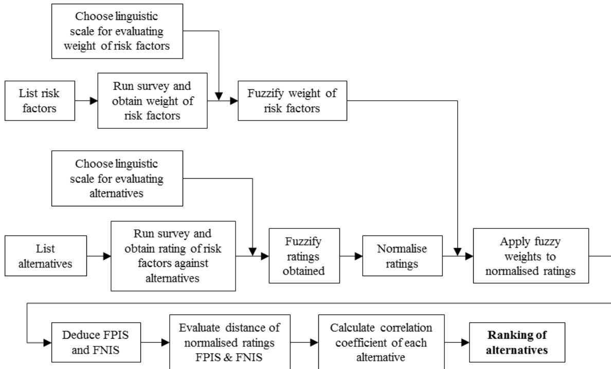
Figure 7. Fuzzy TOPSIS methodology
