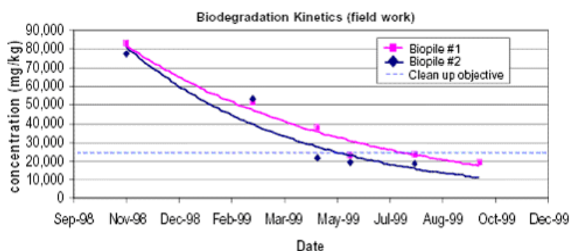
Figure 1: Biopile verification by reference to reductions in TPH load observed in soil (after Berlanger et al. , 2003)
