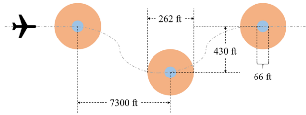
Figure 5. Definition of the slalom task
