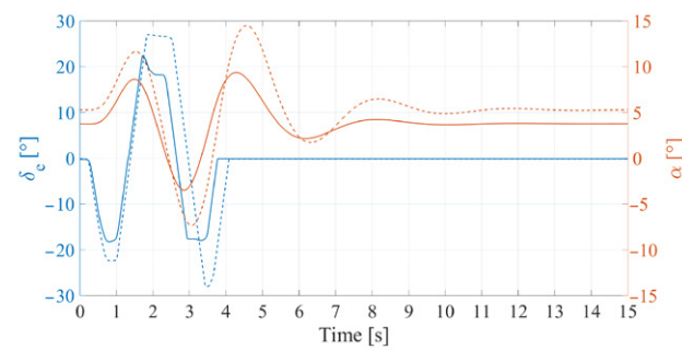
Figure 6. SPPO mode of rigid (–) and flexible (– –) wing aircraft. Here: \delta_e – elevator deflection; \alpha – angle of attack
