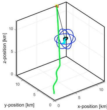
Fig. 5. 3D simulation scenario. The green line represents the UAV trajectory, the blue circumferences represent the safety distance and the cyan line represents the estimated object location obtained from the EKF.
