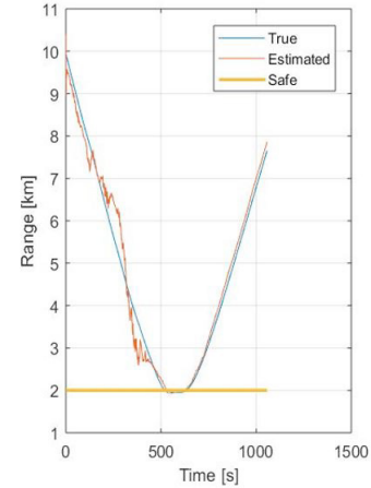
Fig. 6. True and EKF-estimated relative range over time with safety distance.
