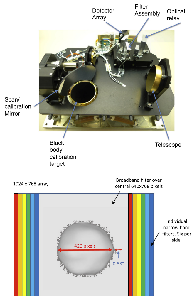
Fig. 9. (Top) The TMC heritage instrument, the Compact Modular Sounder (CMS), flight unit minus its outer cover. CMS has approximate dimensions of 380 \times 335 \times 185 mm. (Bottom) Proposed filter and imaging detector layout, example shown during approach phase to the MBC. The TMC will use an optimised layout, reducing the instrument size to 180 \times 150 \times 120 mm. Mass is 4 kg based on the CMS design.
