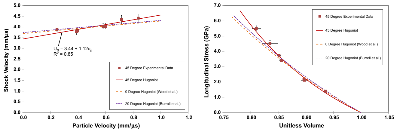
Figure 6 Hugoniot in the U_S – u_p (left) and P – V (right) plane for the 45° orientation of TWCP.
