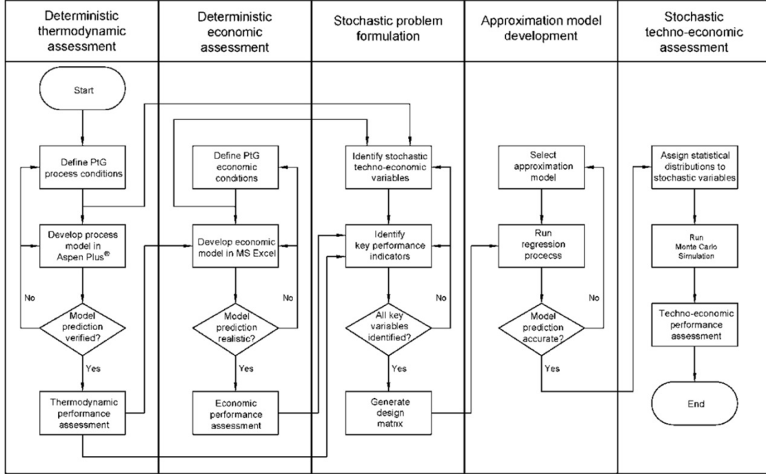
Figure 3: Swim lane diagram for the stochastic techno-economic assessment framework
