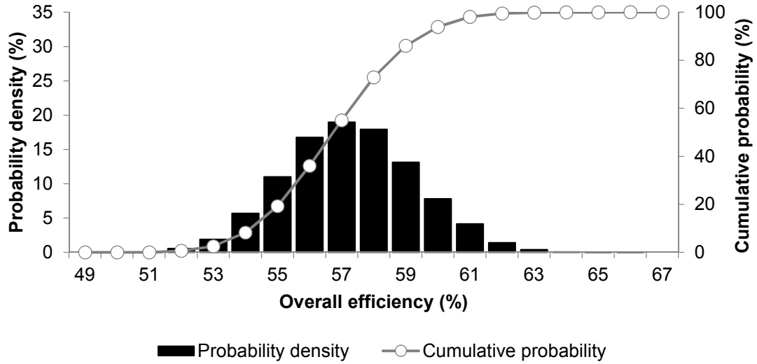
c) Figure 6. Effect of uncertainty on a) heat production, b) heat recovery, and c) overall efficiency of power-to-gas process
