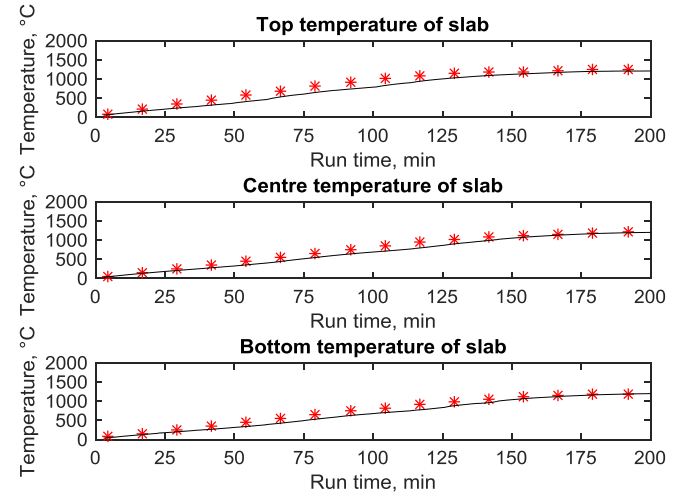
Figure 4. Comparison of the predicted slab heating profile with the desired heating profile (red symbol: predicted profile; black line: desired profile)
