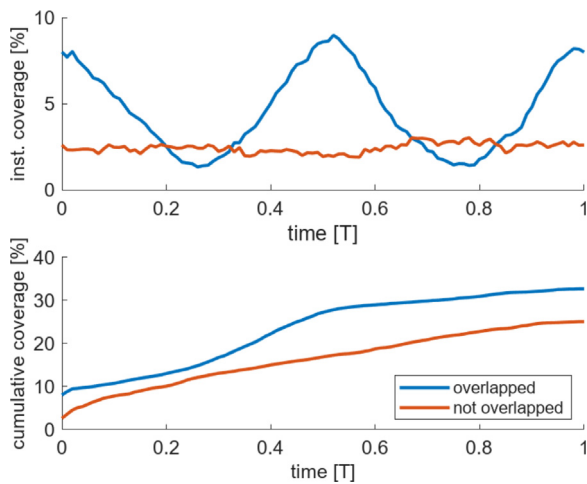
Fig. 27. Comparison of overlapped and non-overlapped low-budget configurations performance, N_{sat/o,L} = 5 . The time is measured as a fraction of the period T of the constellation.
