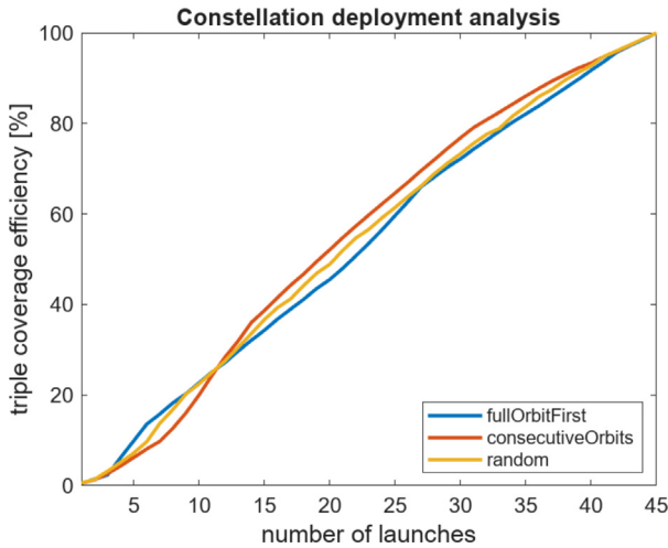
Fig. 24. Comparison of the different deployment strategies for the optimal constellation of Table 5. The triple coverage efficiency is defined as \epsilon_{cov,3} := \frac{cov_{3,deployed}}{cov_{3,full}} .
