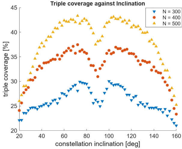
Fig. 18. Triple coverage as a function of the constellation inclination. The fixed constellation parameters are (N_{sat/o}, h, \Omega_0, \Delta\theta) = (50, 460 \text{ km}, 0^\circ, 5^\circ) .
