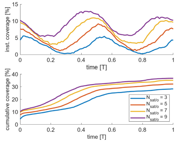
Fig. 28. Performance for varying N_{sat/o,L} , overlapped configuration. The time is measured as a fraction of the period T of the constellation.
