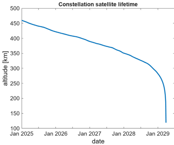
Fig. 10. Natural lifetime of a constellation satellite failure after failure, and thus without manoeuvring capabilities, placed at an altitude of 460 km. Simulation performed with the ESA Drama software [30] using the ECSS-E-ST-10-04C standard for the solar flux [29].
