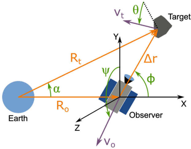
Fig. 3. Diagram of the local reference frame. The displacement vectors have no component along the Z-axis. The observer and target velocity vectors are perpendicular to the Earth–Observer and Earth–Target displacement vectors respectively. Variables are summarised in Table 3.
