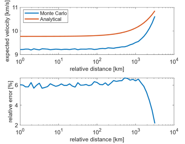
Fig. 5. Analytical estimate for the expected value of the tangential velocity as a function of the relative target–observer distance. Above, a comparison between the analytical estimate and the Monte Carlo simulation. Below, the relative error between the two.
