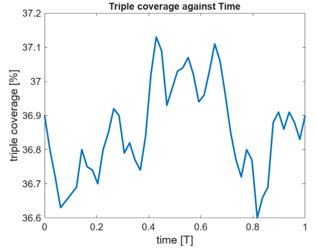
Fig. 13. Time variation of triple coverage. The time is measured as a fraction of the period T of the constellation.
