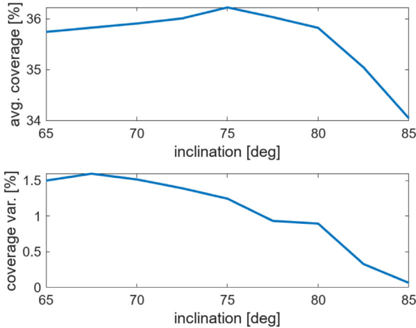
Fig. 16. Yearly triple coverage against constellation inclination, considering only the change in the elevation of the Sun direction. Above, the average yearly triple coverage. Below, the yearly triple coverage variation computed as the difference between the maximum and the minimum coverage.
