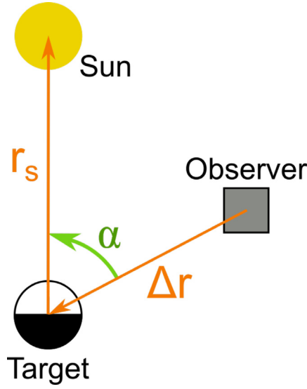
Fig. 7. Phase angle diagram. If \alpha > 90^\circ , more than half of the illuminated part of the target body is not reflecting photons back to the observer, and therefore it is not observable as a first approximation.
