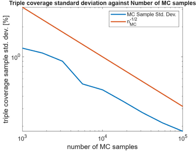
Fig. 12. Triple coverage sample standard deviation against number of Monte Carlo samples.
