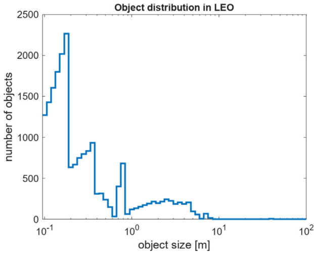
Fig. 29. Target size distribution in LEO as simulated using the ESA Master Software [34]. The y-axis indicates the number of objects per size bin. Notice that the x-axis is in logarithmic scale.
