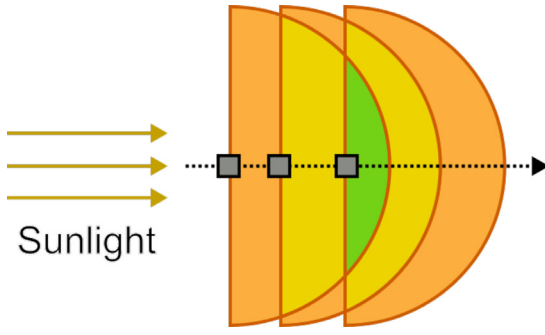
Fig. 9. Example of field-of-regard overlapping for three satellites on the same trajectory. The green area is the triple visibility area.
