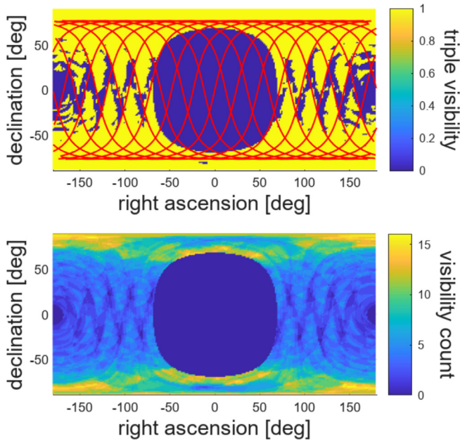
Fig. 21. Visibility map of the optimal constellation in the ECI frame at 550 km altitude during the Autumn equinox. Above, the yellow-shaded area is the area under triple visibility conditions and the red trajectories are the tracks of the constellation. Below, the visibility count for the optimal constellation at 550 km altitude. A visibility count of three or more means that the target is under triple visibility conditions. The large hole at the centre corresponds to the surface area under eclipse conditions.
