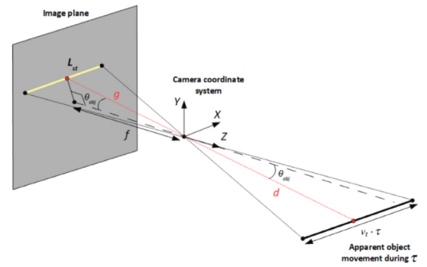
Fig. 1. Pinhole camera model [21].
