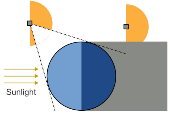
Fig. 8. Possible field-of-regard shapes under the four visibility conditions. The field-of-regard (FOR) is the region where an observation is theoretically possible: when the target is in the orange area, it becomes visible to the observer satellite, represented as a grey square.
