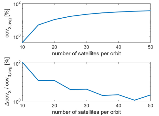
Fig. 14. Time variation of triple coverage against number of satellites per constellation orbit. Above, the mean triple coverage per N_{sat/o} . Below, the ratio between \Delta cov_3 = \max_i(cov_3(t)) - \min_i(cov_3(t)) and the average triple coverage per N_{sat/o} .
