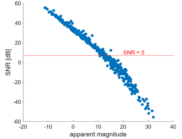
Fig. 2. Signal-to-noise ratio against apparent magnitude for the sensor parameters in Table 1. The curve is retrieved using a Monte Carlo simulation with random target parameters. The resulting limiting magnitude is approximately 12.
