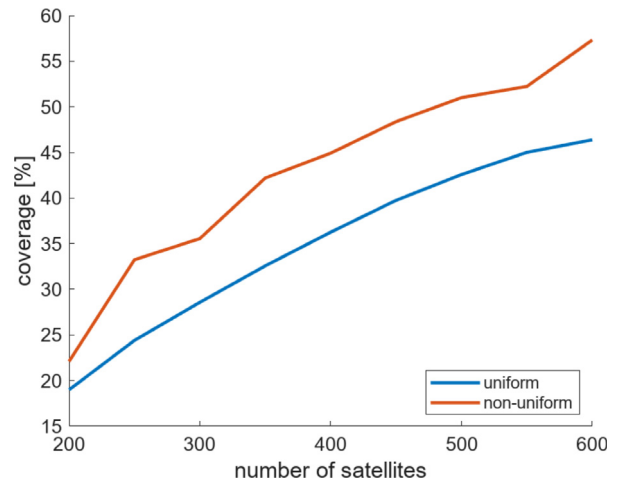
Fig. 32. Triple coverage as a function of the number of constellation satellites. The blue curve considers a uniform target distribution over the LEO region, while the orange one considers the ESA Master estimate shown in Fig. 31. Both cases consider constellation parameters (N_{sat/o}, h, i, \Omega_0, \Delta\theta) = (50, 460 \text{ km}, 70^\circ, 0^\circ, 5^\circ) with variable N_o .
