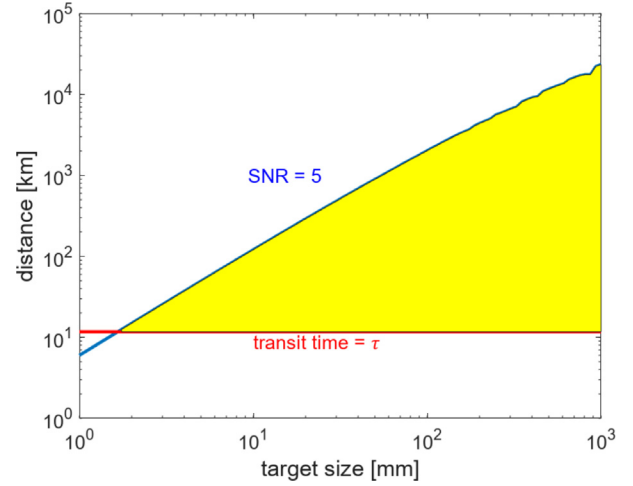
Fig. 6. Maximum observable range against target size. The yellow area is the region for which the target is visible to the observer.
