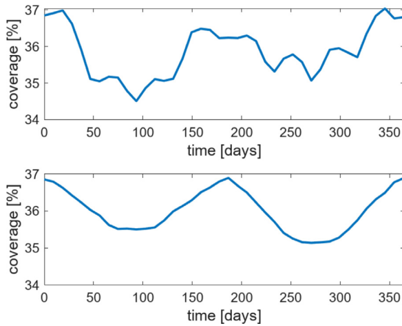
Fig. 15. Yearly triple coverage, varying owing to the variation of the Sun–Earth displacement. Above, the combined effect of the azimuthal and elevation variation of the Sun’s direction. Below, elevation effects only.
