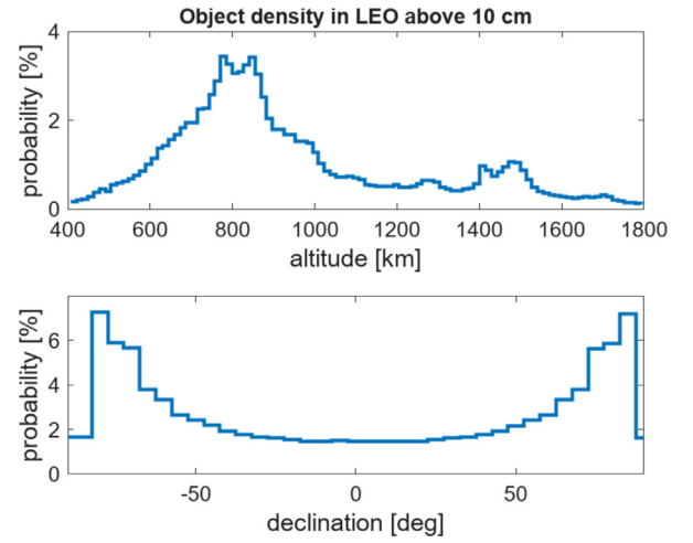
Fig. 31. Target distribution over the LEO region as simulated using the ESA Master Software [34]. The y-axis indicates the probability that a target is in the corresponding altitude or declination bin. This distribution considers targets of size 10 cm or higher.
