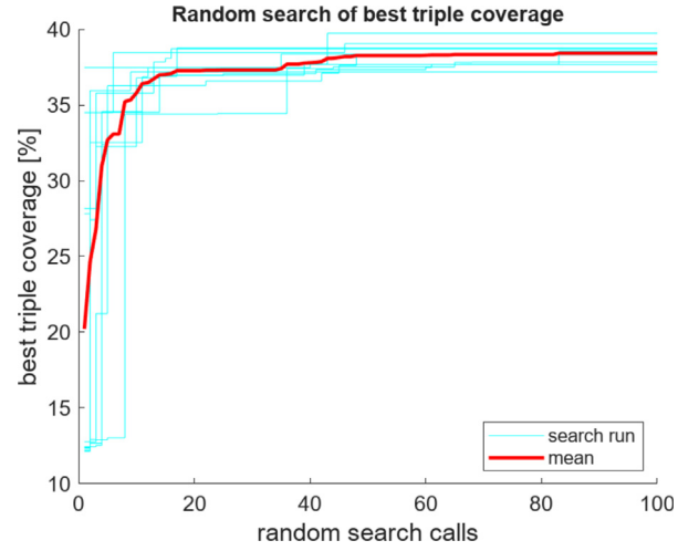
Fig. 19. Constellation optimisation using random search, N = 400 , \Delta N = 5 . In cyan, the single random search runs. In red, their averages. A solution lying near the Pareto front is found on average after only 20 function calls.
