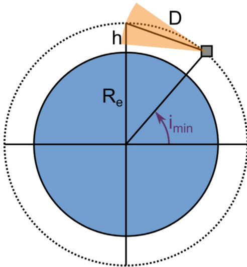
Fig. 11. Diagram of minimum inclination for an observer satellite to be able to see the polar region. D is the maximum range and h is the constellation altitude.
