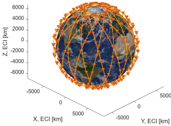
Fig. 20. Optimal constellation. Notice that the constellation is not fixed with respect to the Earth's surface due to the Earth's rotation.
