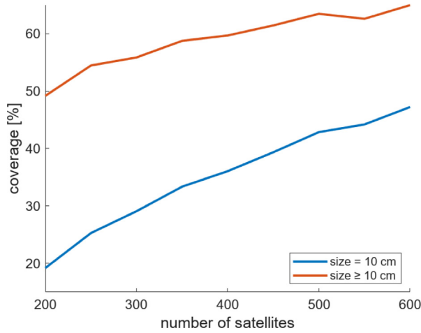
Fig. 30. Triple coverage as a function of the number of constellation satellites. The blue curve considers coverage computed considering only 10 cm targets. The orange curve considers the whole population of size equal or greater than 10 cm. Both cases consider constellation parameters (N_{sat/o}, h, i, \Omega_0, \Delta\theta) = (50, 460 \text{ km}, 70^\circ, 0^\circ, 5^\circ) with variable N_o .
