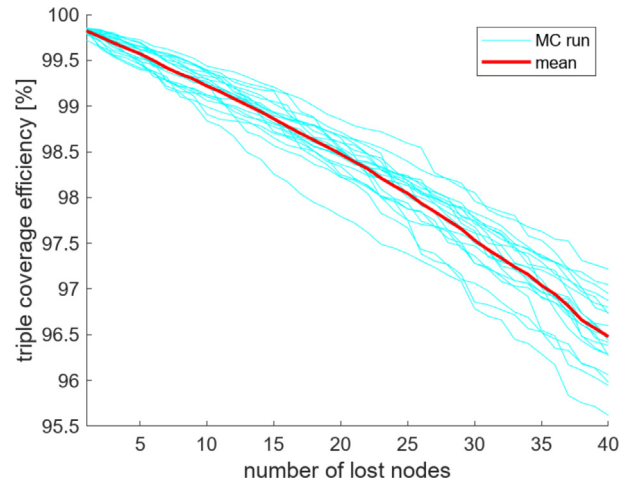
Fig. 22. Satellite loss analysis for random satellite loss in the optimal constellation of Table 5. In cyan, single Monte Carlo runs. In red, the average satellite loss behaviour. The triple coverage efficiency is defined as \epsilon_{cov,3} := \frac{cov_{3,surv}}{cov_{3,healthy}} .
