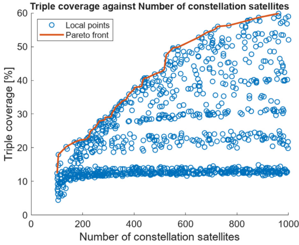
Fig. 17. Tradespace exploration. Each point corresponds to a specific set of parameters sampled randomly from the search space. The band structure is due to the integer nature of the N_o and N_{sat/o} parameters. For instance, the first band from below corresponds to N_o = 1 . In orange, the Pareto front for the constellation architecture. Notice that the front is just an estimate based on random assignment, and therefore it is an underestimation of the actual front.
