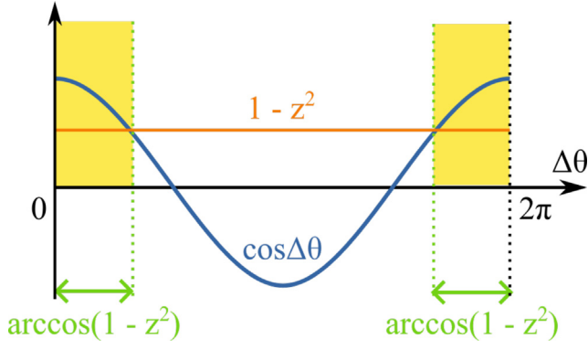
Fig. 4. The yellow-shaded area is the region for which \cos \Delta\theta \geq 1 - z^2 . The total length of the region on the [0, 2\pi] interval is 2\arccos(1 - z^2) .
