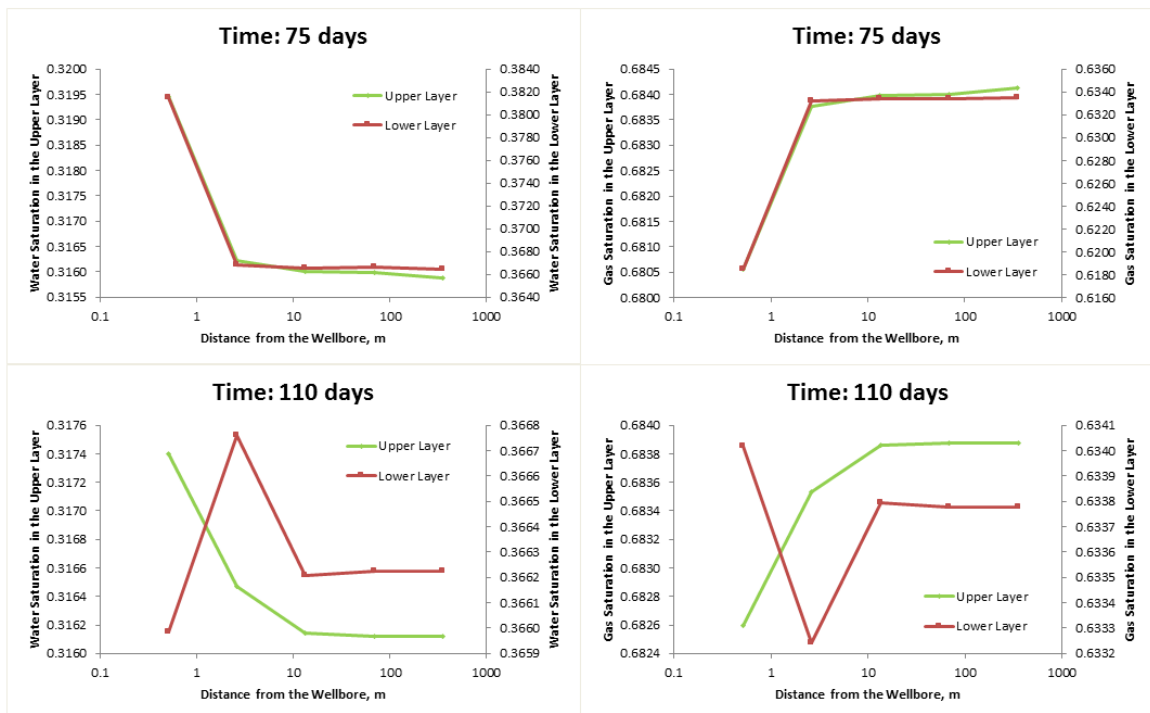
Fig. 16 – Saturation profiles along the near-wellbore region at different points in time during the second shut-in period. The horizontal axis captures the distance from the wellbore center to the logarithmic center point of each block.
