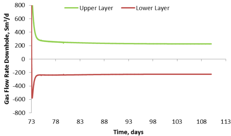
Fig. 15 – Gas flow rates at the inner boundary during the second shut-in period.
