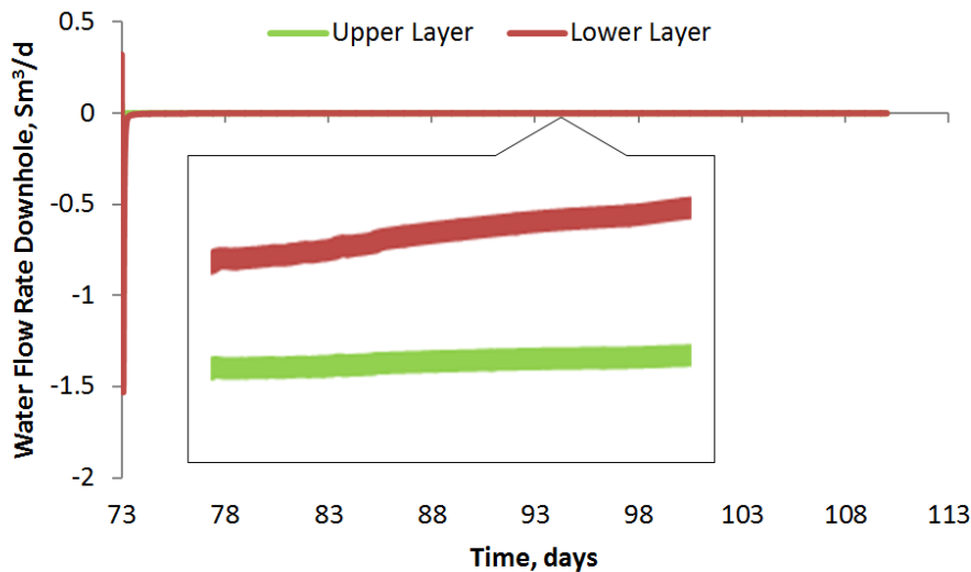
Fig. 14 – Water flow rates at the inner boundary during the second shut-in period.
