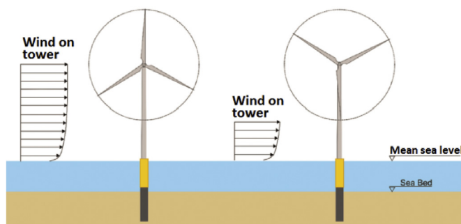
Fig. 2. Cyclic/dynamic load acting on the tower due to blade shadowing effect (3P load).
