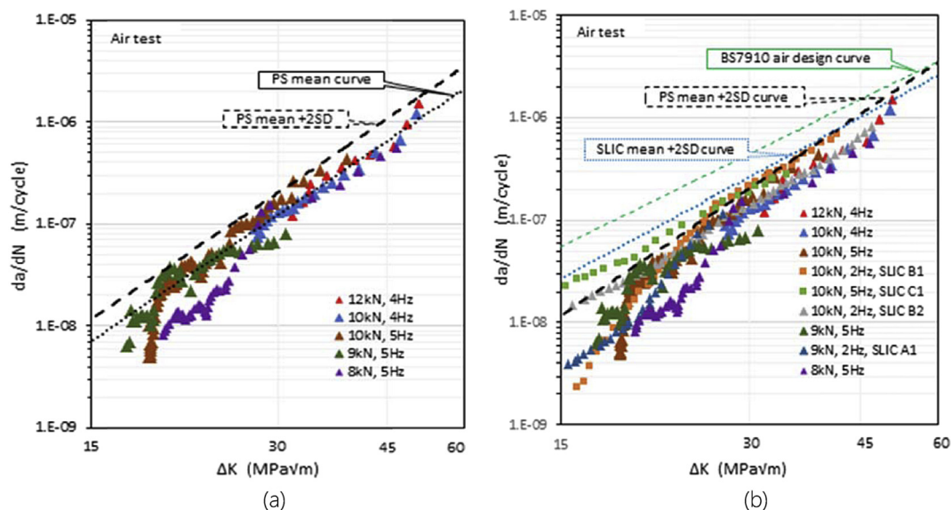
Fig. 9. FCGR in air (a) for S355G10 + M in the present study (b) Comparison of S355G10 + M with S355G8 + M in the SLIC study.
