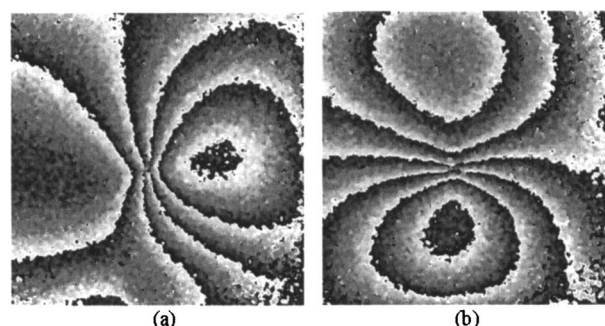
Fig. 2 The wrapped phase maps, determined using the shearography technique, for (a) a horizontal shear of 2.5 mm and (b) a vertical shear of 2.5 mm.
