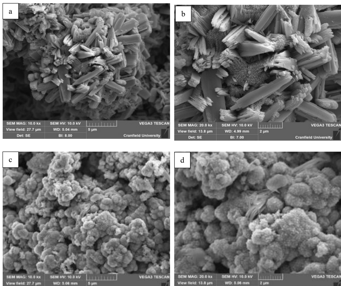
Figure 16 SEM micrographs (at 10kx and 20kx) of corrosion product from J-series steel coupons recovered after (a, b) 105 days (c, d) 227 days of immersion in nitrated artificial seawater
