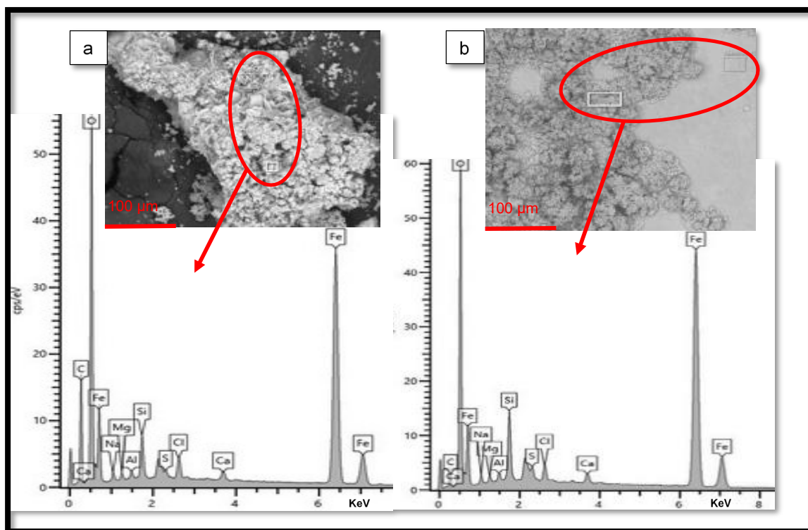
Figure 13 EDS results for corrosion products collected from anodic regions of C-series steel coupons immersed in artificial seawater for 321 days
