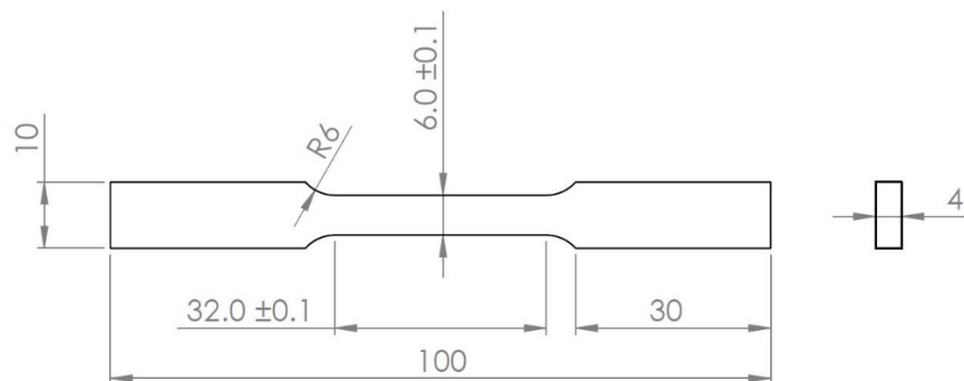
Figure 5: Dimensions (in mm) of the tensile specimens used for RT tensile testing, conforming to ASTM E8/E8M subsize standard.
