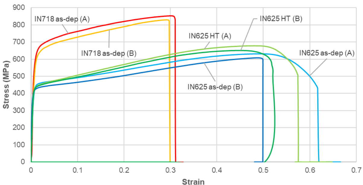
Figure 13: RT Stress vs. Strain for as-deposited IN718, IN625 & Heat-treated (HT) IN625. Best (A) and worst (B) performing samples are shown in each category.
