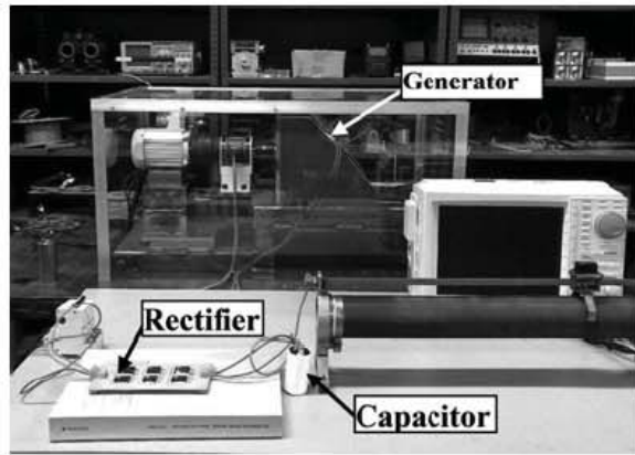
Figure 11 Experiment setup
