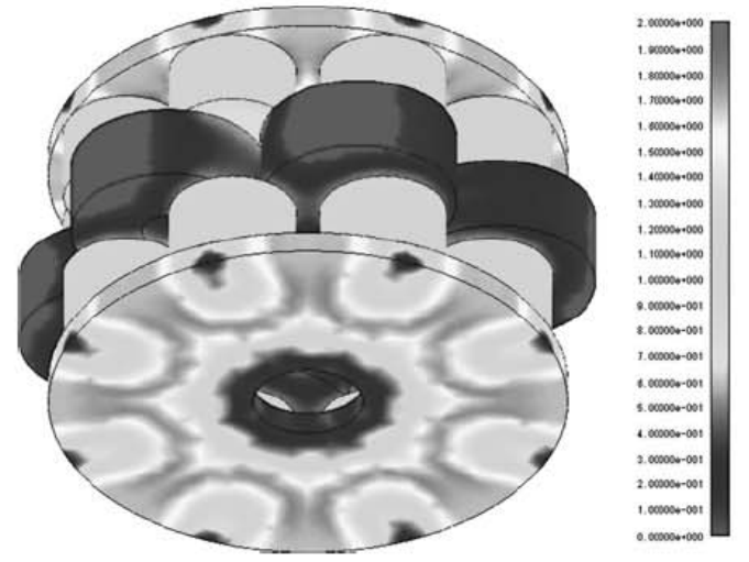
Figure 4 No-load magnetic flux density distribution in the machine
