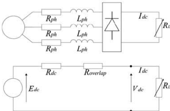
Figure 2 DC resistive load circuit and the equivalent circuit
