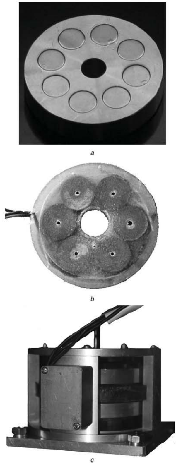
Figure 10 Prototype machine
