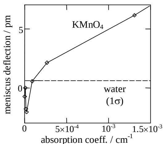
Figure 8. Photothermal meniscus deflection results excited by a 658nm LED, following subtraction of the mean measured meniscus deflection for a deionised water control.
