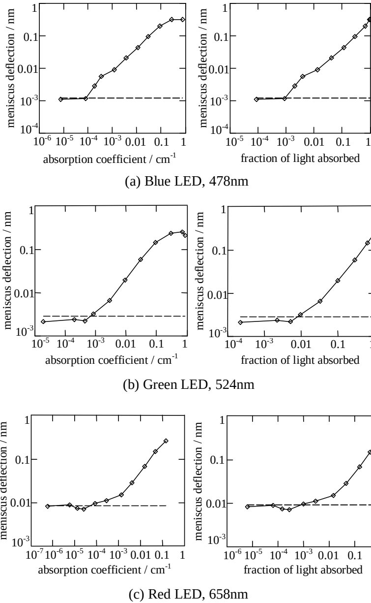
Figure 7. Photothermal signals from \text{KMnO}_4 solutions (solid line) and from deionised water controls (dashed line), versus the absorption coefficients and fractional light absorption of \text{KMnO}_4 at each wavelength.
