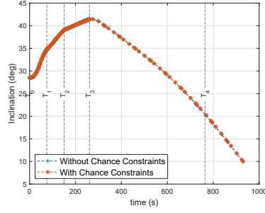
(c) Inclination
