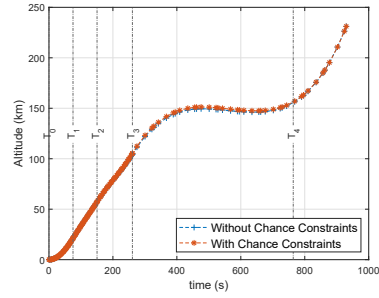
(f) Attitude
