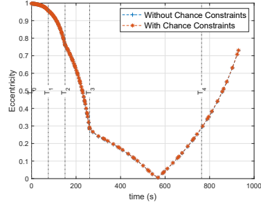
(b) Eccentricity
