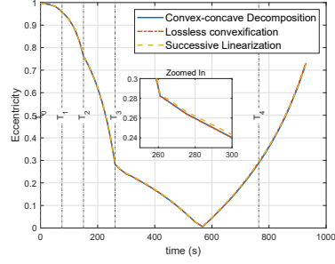
(b) Eccentricity
