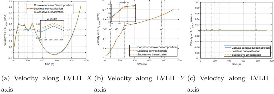
Figure 5: The velocity comparing results under LVLH frame
