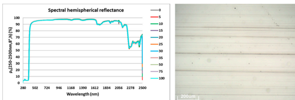
Figure 4. Hemispherical reflectance after 100 cycles and scratches after 10 cycles (cleaning abrasion test).
