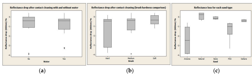
Figure 12. Reflectance drop as measured on the D&S, shown in comparison to the presence of (a) water; (b) brush hardness and (c) sand type.
