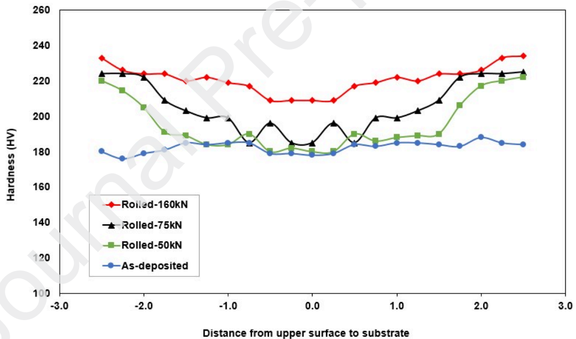
Fig. 8. Effect of rolling load P(\text{kN}) and hardness variation across the through thickness direction (rolling on both surfaces)
