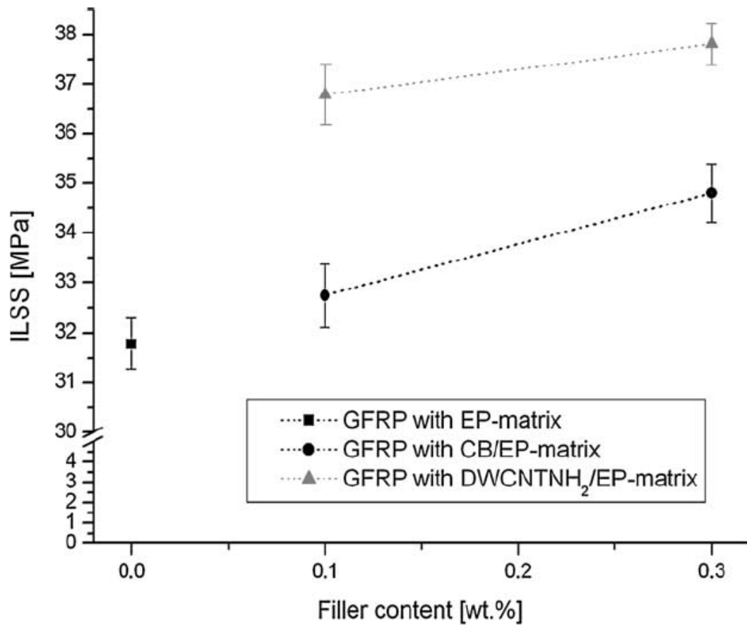
Figure 2 Interlaminar shear strength (ILSS) of the (nano-reinforced) GFRPs (EP-epoxy, CB- carbon black and DWCNT – double wall carbon nanotubes) [57].
