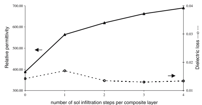
Fig. 4 Variation in relative permittivity and dielectric loss of 4[\text{C} + \text{xS}] as a function of sol infiltration
