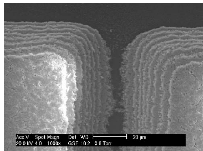
Fig. 11 SEM micrograph of a 21-μm PZT thick film patterned with features of 10 μm at the base
