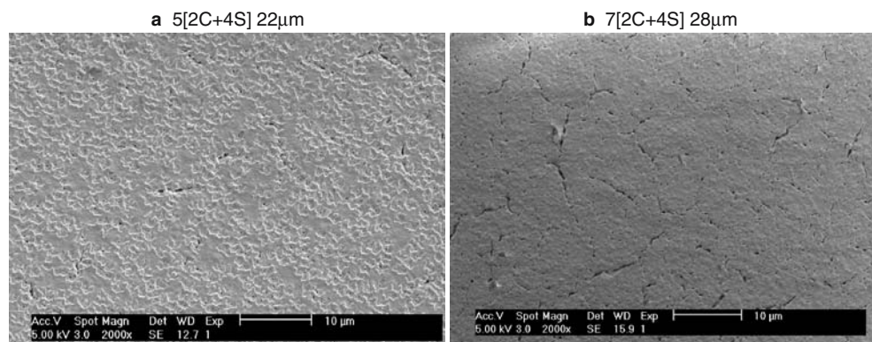
Fig. 8 SEM micrograph of surface finish of the process x [2C+4S] for two different thicknesses of film showing a marked reproduction in cracking in comparison to x[C+4S] films. a Shown with 100 nm of Pt sputtered the surface. b Virgin PZT surface
