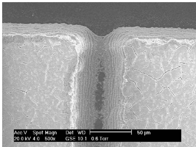
Fig. 12 SEM micrograph of a 30- \mu m PZT thick film patterned with features of 50 \mu m at the surface and 10 \mu m at the base
