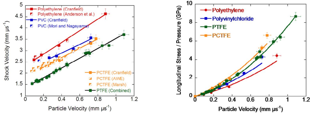
a. Shock velocity – particle velocity b. Stress – particle velocity Fig. 4. Hugoniot of polymers under investigation.
