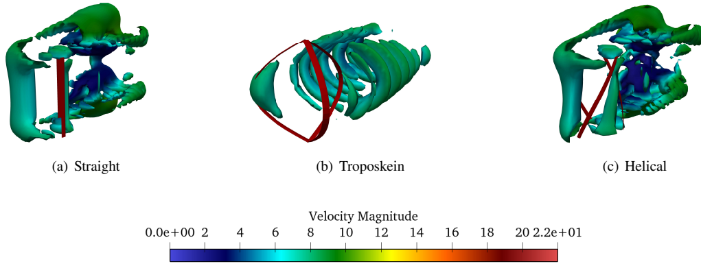
Fig. 10 Instantaneous 3D flowfield using iso-surfaces of the Q criterion for vortices visualization, using mid-fidelity LLFVW, at TSR = 3.3
