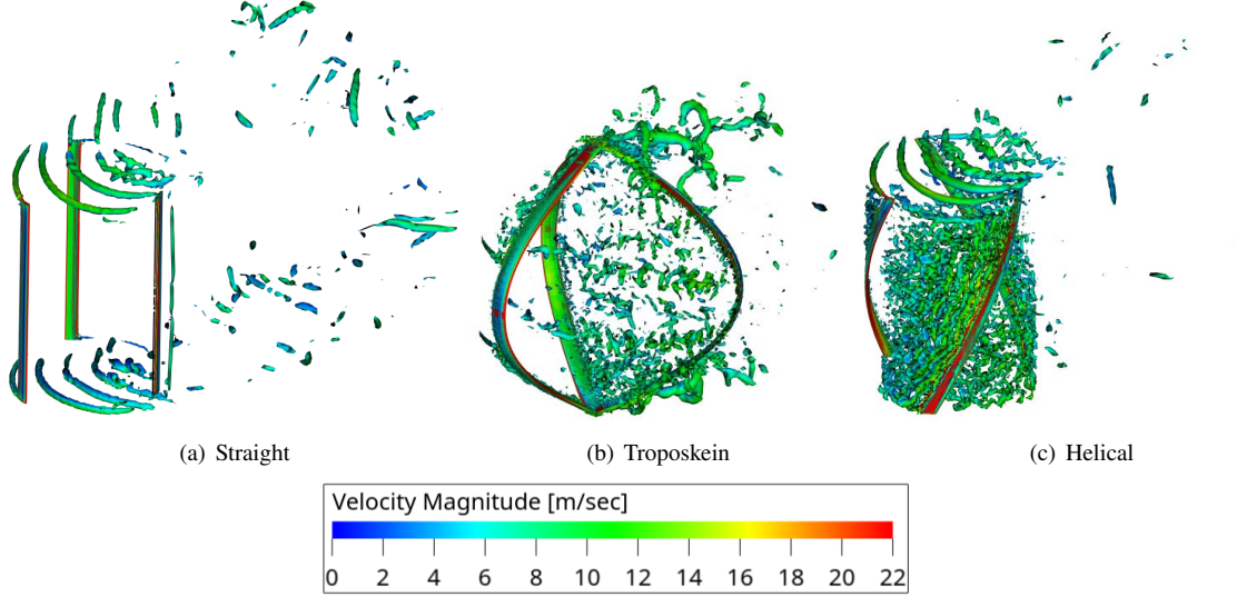
Fig. 9 Instantaneous 3D flowfield using iso-surfaces of the \lambda_2 criterion for vortices visualization, using high-fidelity LBM, at TSR = 3.3
