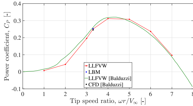
Fig. 5 C_P values for a range of \text{TSR} using QBlade and for \text{TSR} = 3.3 using PowerFLOW for the 1-bladed Darrieus VAWT; comparison is made with results from Balduzzi[11]
