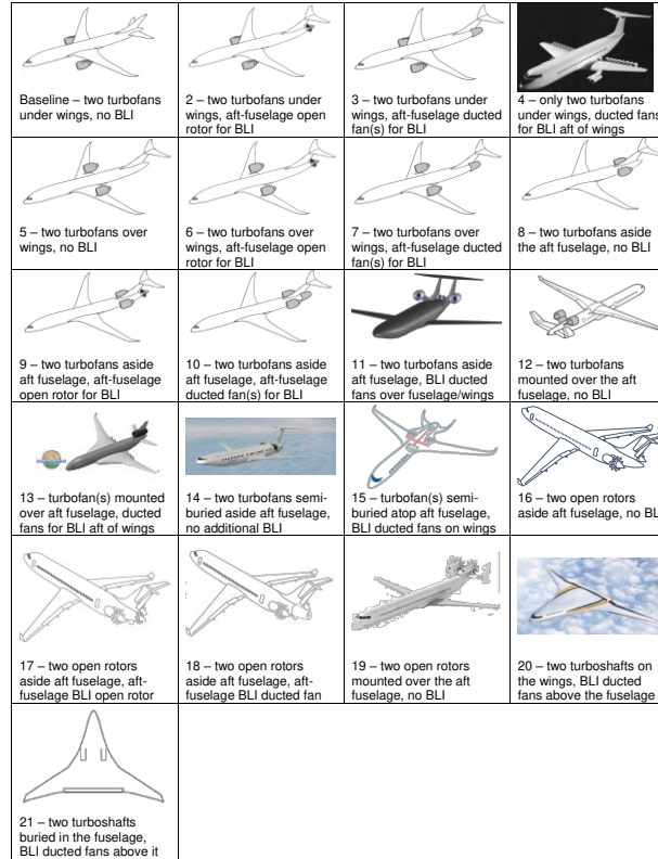
FIGURE 10: Propulsion systems configuration assessed in the first phase of the down-selection
