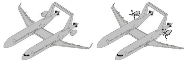
FIGURE 2: Left, SMR CU1. Right SMR Chalmers
