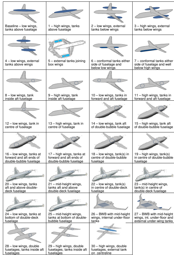
FIGURE 9: Airframe configurations assessed in the first phase of the down-selection
