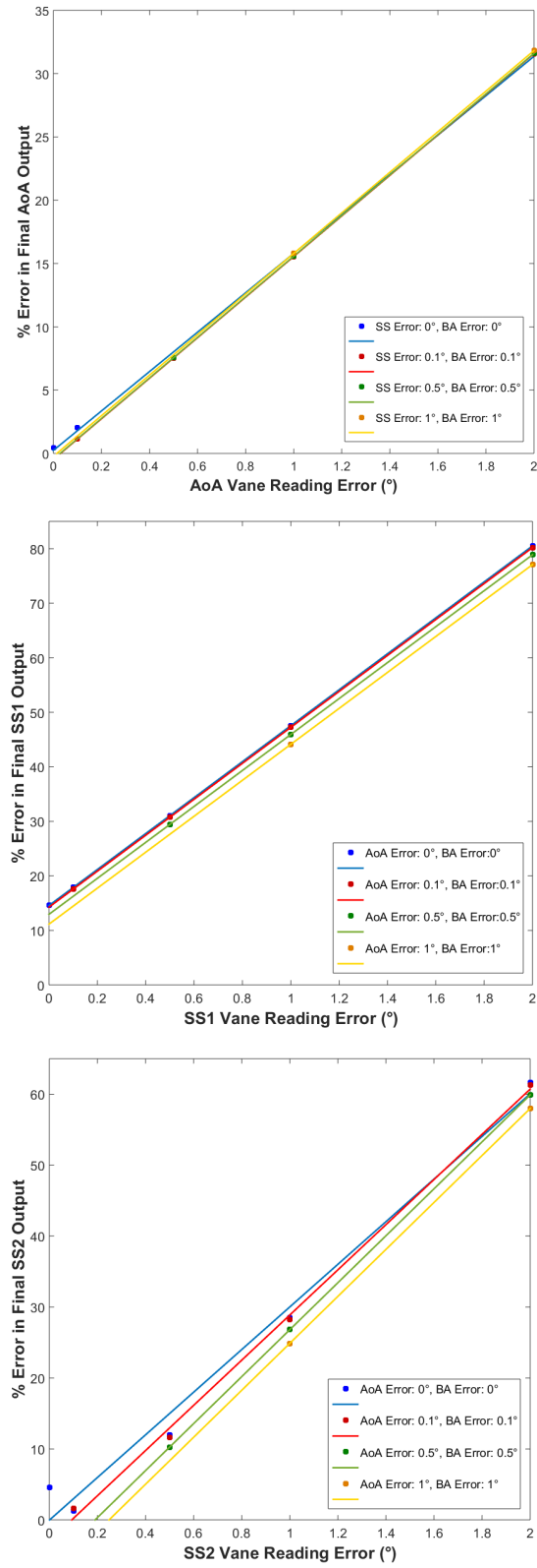
Figure 15: Propagation of input errors throughout the calibration method and correction.
