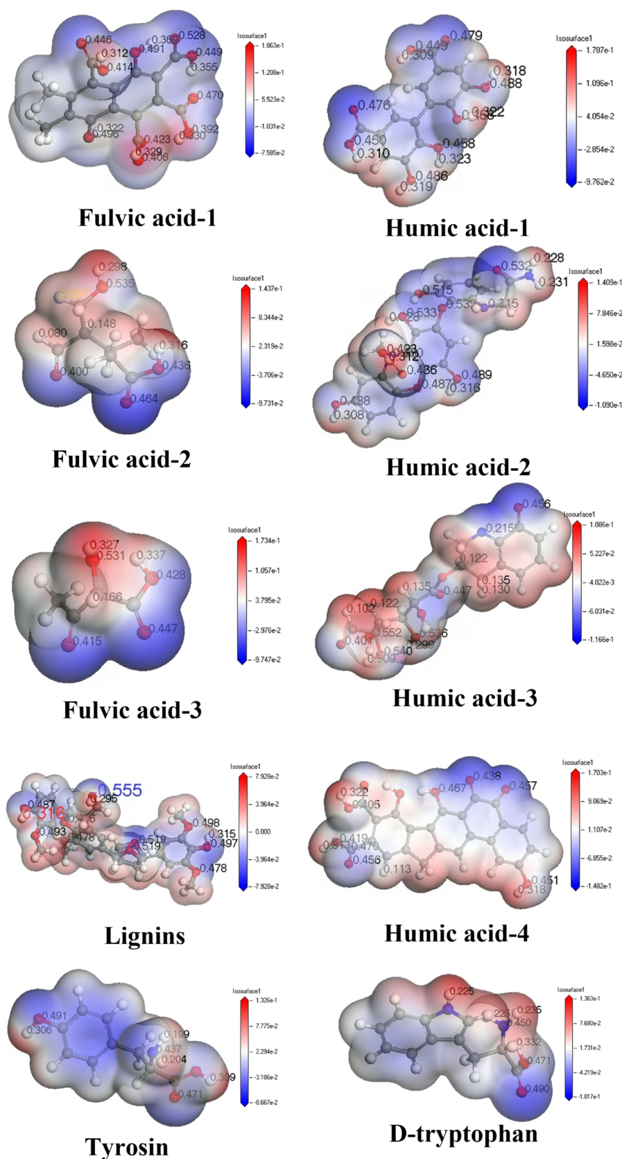
Fig. 6. Molecular structural, electron clouds and single-point charge diagrams of model organic substance structures. The blue and red color represents the positive and negative electron clouds, respectively. The shade of the color represents the change in charge density.
