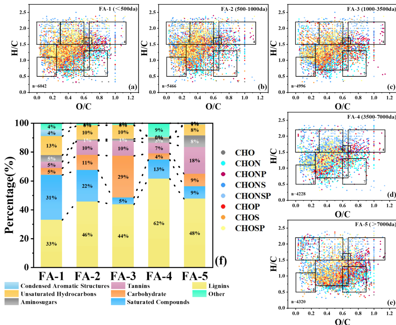
Fig. 5. Van Krevelen diagram of FA-1 (a), FA-2 (b), FA-3 (c), FA-4 (d) and FA-5 (e). The rectangles indicate regions associated with lipids (1), proteins (2), aminosugars (3), carbohydrates (4), condensed hydrocarbons (5), lignin (6), and tannin (7); Proportional distributions of identified molecules in each FA samples (f).
