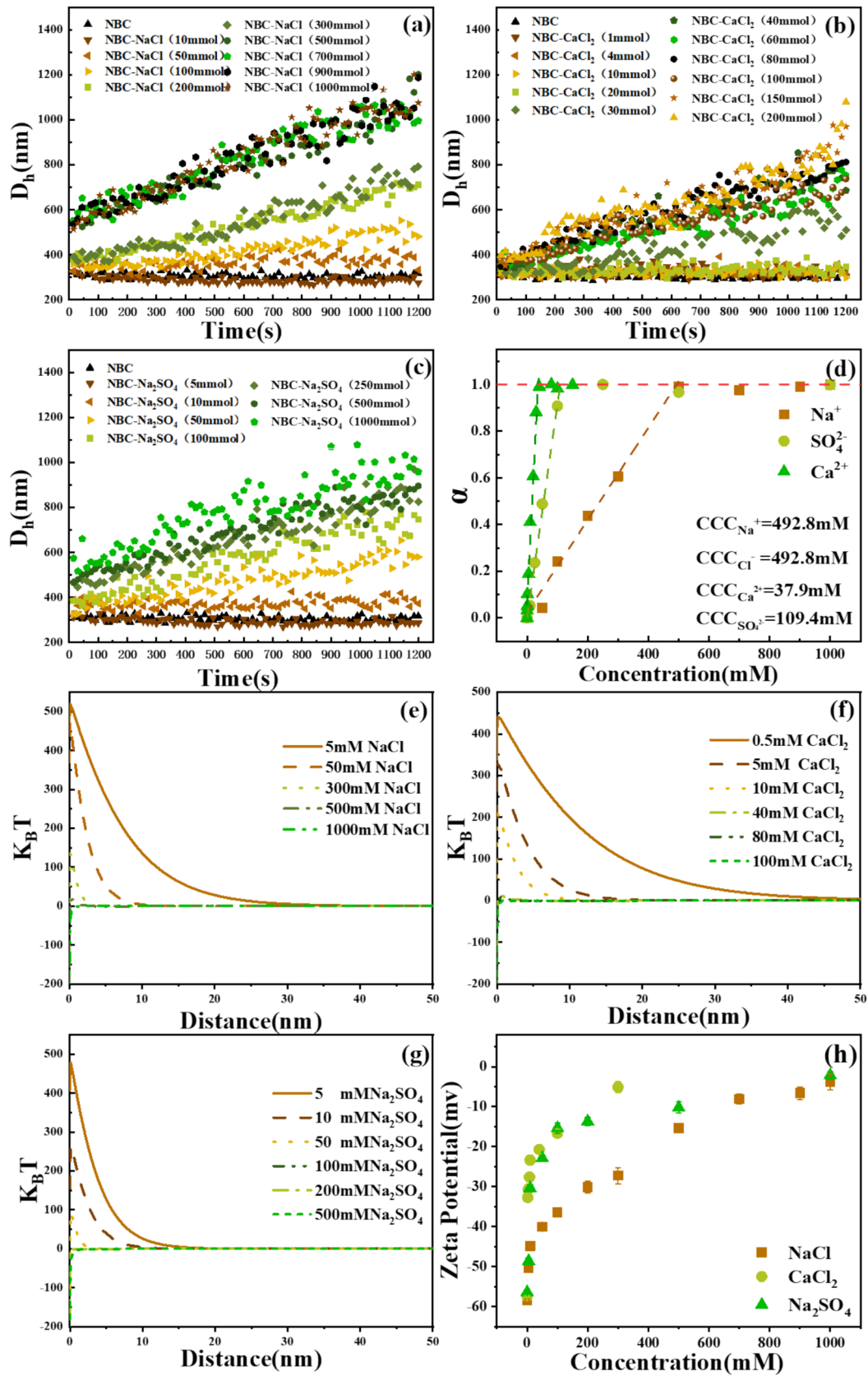
Fig. 1. Hydraulic diameters ( D_h ) of NBC in NaCl (a), CaCl_2 (b), and Na_2SO_4 (c) solutions with varying ion concentrations; Critical coagulation concentration (CCC) of NBC in different ion solutions (d); Relationship between normalized DLVO interaction energy ( K_B T ) curve and separation distance of NBC in NaCl (e), CaCl_2 (f), and Na_2SO_4 (g) solutions; Zeta potential of NBC in different ion solutions (h).
