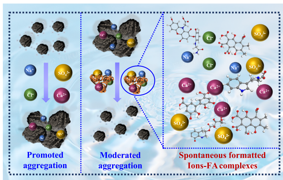
Fig. 7. Schematic diagram of the NBC aggregation in the presence of ions and moderated by aromatic components in DOM.
