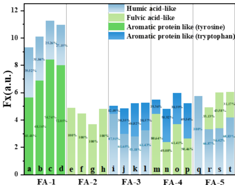
Fig. 4. Identified organic components in FA-1 (a), FA-2 (e), FA-3 (i), FA-4 (m), and FA-5 (q) samples; Identified organic components of NBC-ions-FA solutions after the aggregation experiments. In which, FA-1 (b), FA-2 (f), FA-3 (j), FA-4 (n), FA-5 (r) are in \text{CaCl}_2 solutions; FA-1 (c), FA-2 (g), FA-3 (k), FA-4 (o), FA-5 (s) are in \text{Na}_2\text{SO}_4 solutions; and FA-1 (d), FA-2 (h), FA-3 (l), FA-4 (p), FA-5 (t) are in \text{NaCl} solutions.
