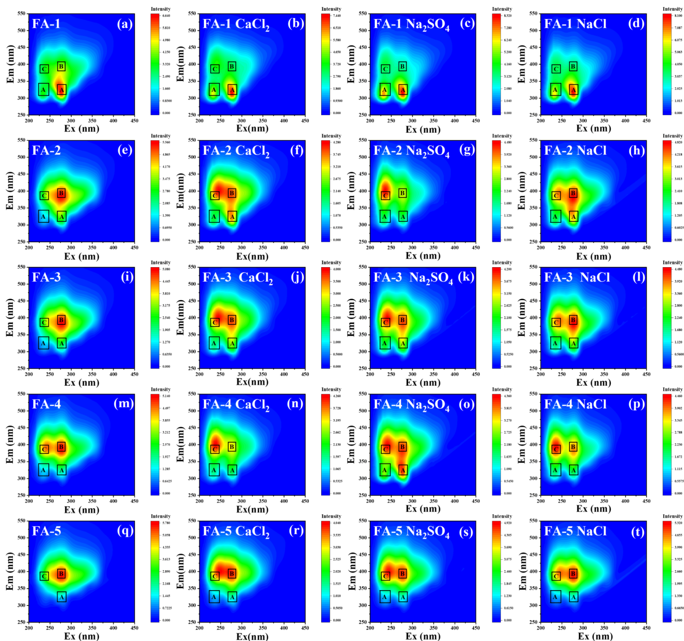
Fig. 3. Piloted three-dimensional fluorescence spectra of FA sample with five MWs, FA-1 (a), FA-2 (e), FA-3 (i), FA-4 (m), FA-5 (q); Piloted three-dimensional fluorescence spectra of NBC-ions-FA after the aggregation experiments. The corresponding solution matrix was marked at the top of each spectra map. For example, FA2 CaCl 2 (f) represents the spectra of the NBC-CaCl 2 -FA-2 solution after the aggregation experiment.
