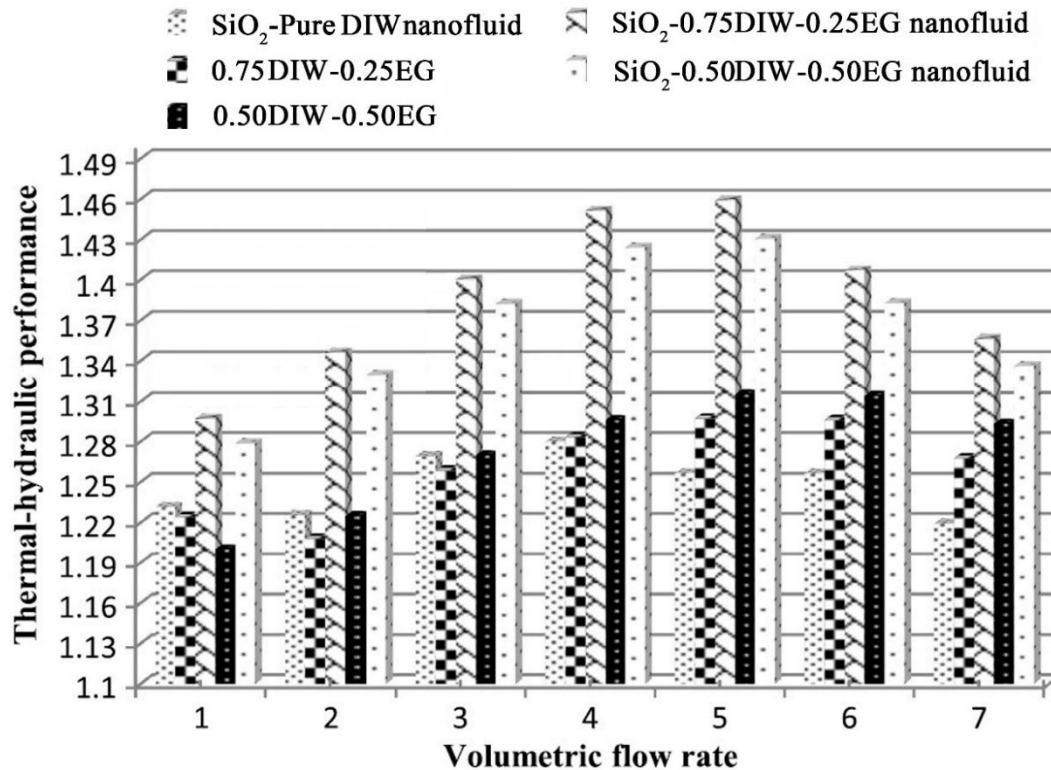
Figure 19. Variations of the thermal-hydraulic performance versus volumetric flow rate for different ratios of DIW-EG mixture as the basefluid for the \text{SiO}_2 -based nanofluid [206].
