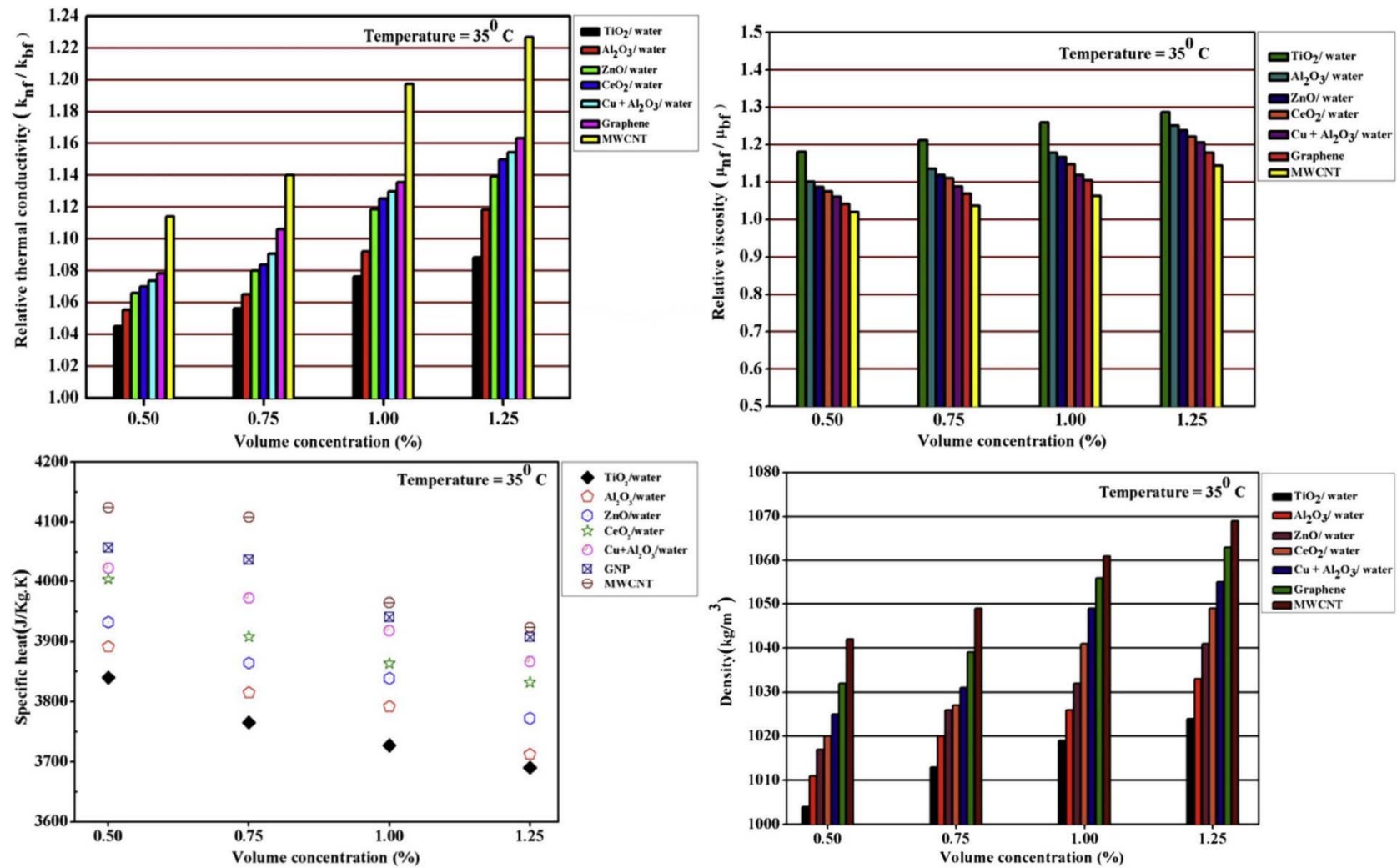
Figure 12. Variation of the relative thermophysical properties of the studied nanofluids. Reproduced with permission from [183]. Elsevier, 2016.
