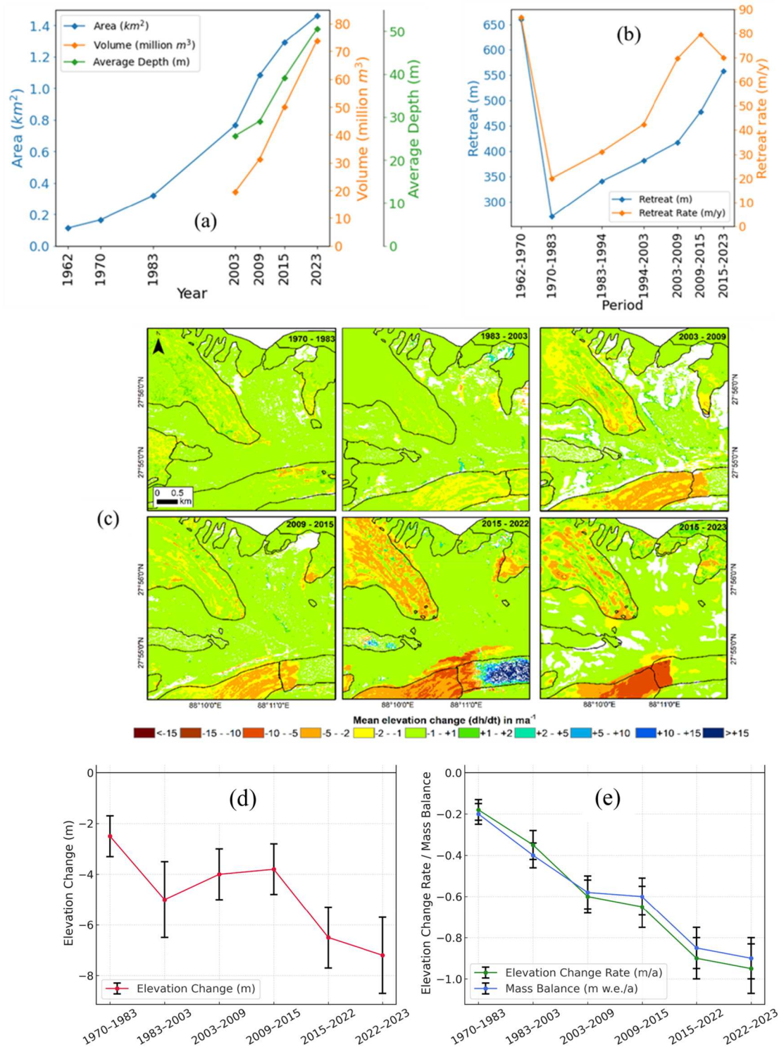
Figure 2. (a) Area change (1962–2023), volume change (2003–2023) and average depth of the lake change (2003–2023), (b) Retreat distance (1962–2023) and rate of retreat of the glacier between 1962 and 2023, (c) Surface elevation change rate (m/a), showing the spatial distribution around SLG, highlighting glacier retreat and lake expansion over time, (d) temporal elevation change trends observed for various time intervals from 1970 to 2023, and (e) mass balance and elevation change rate, from 1970 to 2023.
