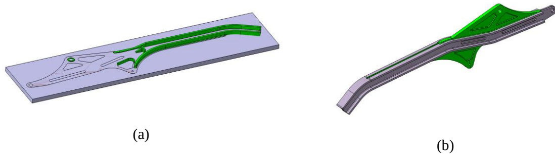
Figure 13. Alternative Design Solutions for Flap Track (a) WAAM Deposition on Thick Plate (b) WAAM Deposition on Formed Extrusion (WAAM Deposition Shown in Green)
