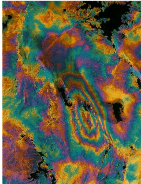
Figure 2: Surface displacement associated with the May 17, 1993 Eureka Valley earthquake in a remote section of eastern California, measured interferometrically using data from ERS-1. One fringe represents 28 mm of range change. Concentric rings just below the image's centre show subsidence of up to 9.5 cm [2].
