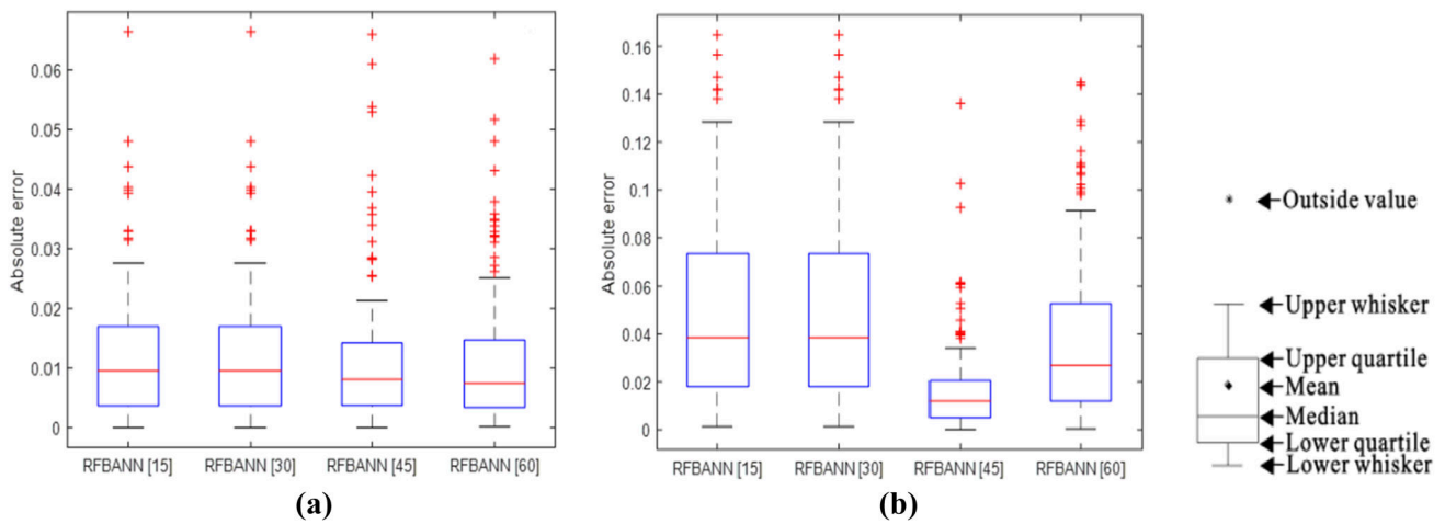
Fig. 34 Boxplots of absolute errors for RBFANN models for: a M-04 (no swirl) and b M-09 (swirl flow)
