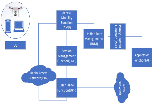
Fig. 1 System Architecture for fifth generation networks
