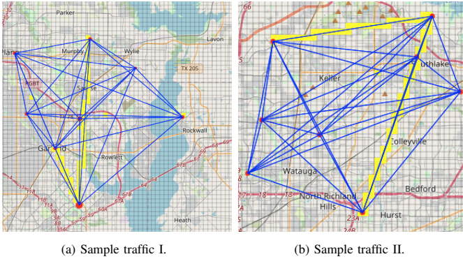
Figure 2. Different sample traffics with different sizes that are generated around Dallas - Fort Worth area including both strategic and pre-tactical conflict cases. Vertiports are in red, routes are in blue, and conflicts are given in yellow. Cell size of the grid map is 500 m. as length and 50 m. as height.
