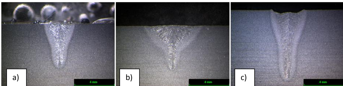
Figure 2: Macrographs of welds obtained at a constant travel speed of 2 m/min; a) laser 4 kW (120 J/mm); b) hybrid 7 kW (210 J/mm); c) laser 7 kW (210 J/mm)
