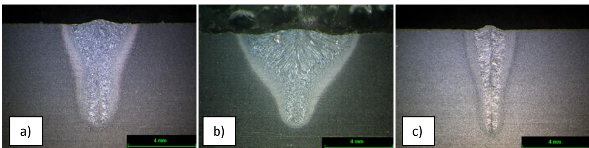
Figure 5: Macrographs of welds of three processes with the combination of parameters required for 6 mm of penetration depth: a) laser welding 4 kW, 1m/min (240 J/mm); b) hybrid welding 7 kW, 1 m/min (420 J/mm); c) laser welding 7 kW, 3 m/min (140 J/mm)
