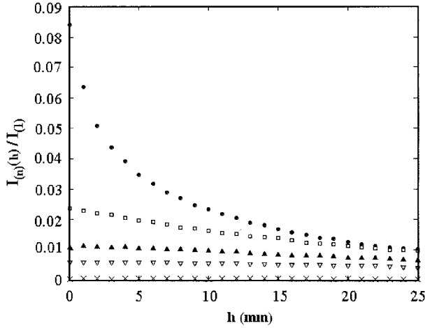
Fig. 4. Intensity of different scattering orders I_{(n)} as a function of h : \bullet , double scattering I_{(2)} ; \square , triple scattering I_{(3)} , \blacktriangle , fourth-order scattering I_{(4)} ; \nabla , fifth-order scattering I_{(5)} , and \times , tenth-order scattering I_{(10)} . The intensity of each scattering order is normalized to the intensity of single scattering I_{(1)} at h = 0 .
