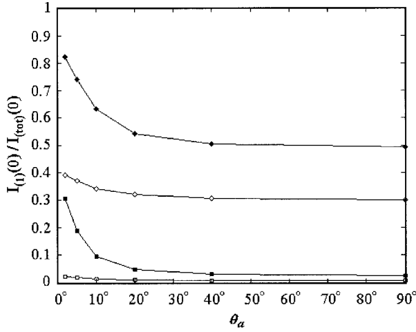
Fig. 10. Results of I_{(1)}/I_{(tot)} versus acceptance angle \theta_a for anisotropic scattering with \beta = 10^\circ and with different scattering coefficients: \diamond , \mu_s = 0.04 \text{ mm}^{-1} for particle diameter a = 15 \text{ }\mu\text{m} ; \square , \mu_s = 0.16 \text{ mm}^{-1} for particle diameter a = 15 \text{ }\mu\text{m} ; \square , \mu_s = 0.04 \text{ mm}^{-1} for particle diameter a = 1 \text{ }\mu\text{m} ; \blacksquare , \mu_s = 0.16 \text{ mm}^{-1} for particle diameter a = 1 \text{ }\mu\text{m} .
