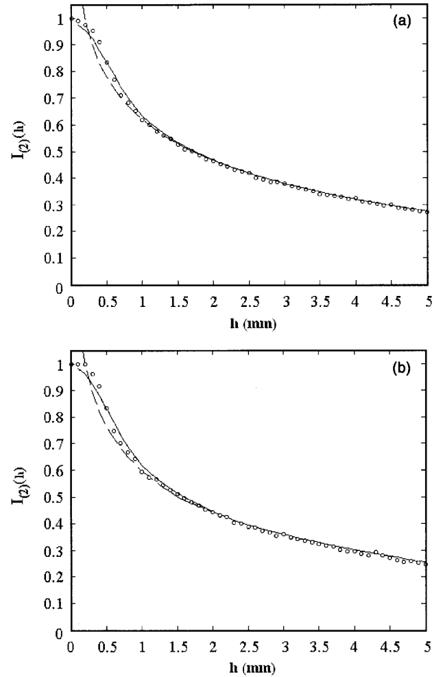
Fig. 3. Intensity of the double light scattering I_{(2)} with respect to the distance h between V_1 and V_2 : (a) \mu_s = 0.04 \text{ mm}^{-1} , (b) \mu_s = 0.16 \text{ mm}^{-1} . The solid curve represents the results of calculation by the exact Eq. (7), the dotted curve by the approximate Eq. (13), and (○) are the results of the MC simulation.
