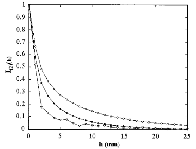
Fig. 7. Normalized intensity of the double light scattering I_2 with respect to the distance h between V_1 and V_2 : \circ , isotropic scattering with \mu_s = 0.04 \text{ mm}^{-1} ; \bullet , isotropic scattering with \mu_s = 0.16 \text{ mm}^{-1} ; \nabla , anisotropic scattering with \mu_s = 0.04 \text{ mm}^{-1} for particle diameter a = 15 \text{ }\mu\text{m} .
