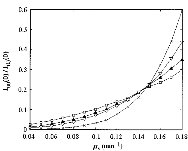
Fig. 6. Normalized intensities of n th scattering orders and single-scattering intensity at h = 0 , I_n(0)/I_1(0) as a function of scattering coefficient \mu_s : \square , triple scattering I_3 ; \triangle , fourth-order scattering I_4 ; \nabla , fifth-order scattering I_5 ; \times , tenth-order scattering I_{10} .
