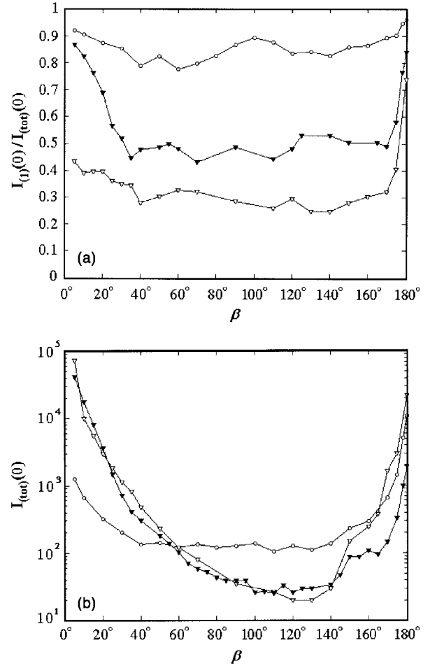
Fig. 9. Effect of the source–detector angle \beta on the single-scattering detection at h = 0 with an acceptance angle of 2^\circ : \diamond , isotropic scattering with \mu_s = 0.04 \text{ mm}^{-1} ; \nabla , anisotropic scattering with \mu_s = 0.04 \text{ mm}^{-1} for particle diameter a = 15 \mu\text{m} ; \blacktriangledown , anisotropic scattering with \mu_s = 0.04 \text{ mm}^{-1} for particle diameter a = 1 \mu\text{m} . (a) Amount of single scattering I_1/I_{tot} detected versus \beta . (b) Total intensity detected versus \beta .
