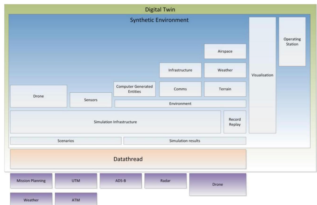
Figure 4. Functional Architecture.
