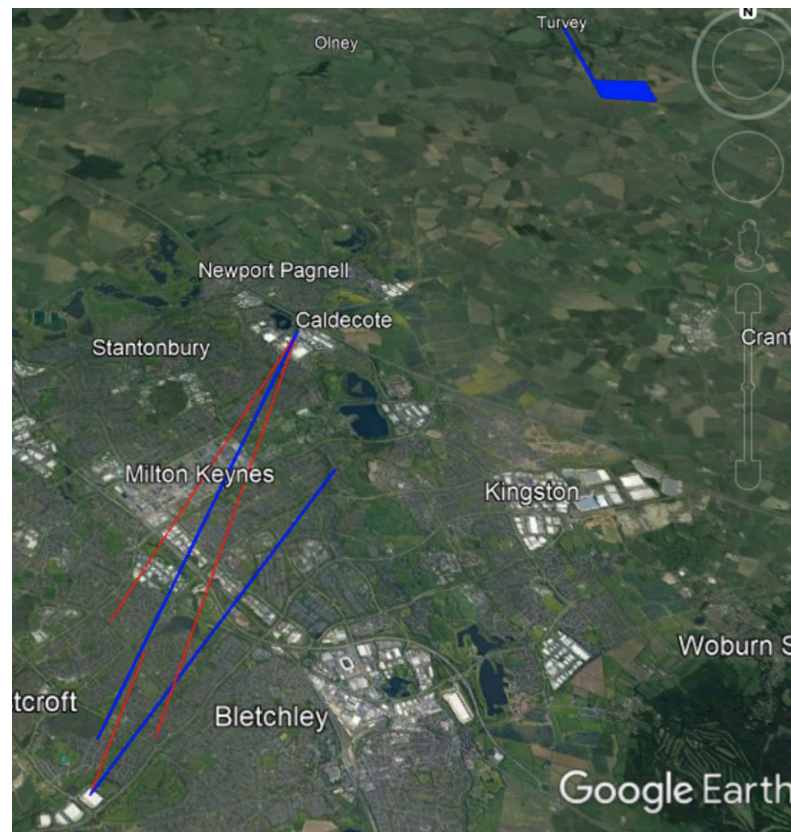
Figure 20. Planned operations for run #4 (Digital Twin flights only)—rejected flights in red.
