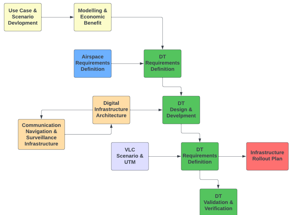
Figure 1. Development process of the digital twin.
