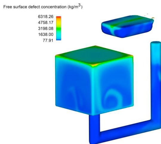
Figure 5: Free surface defect concentration (Basic Gating System Design)
