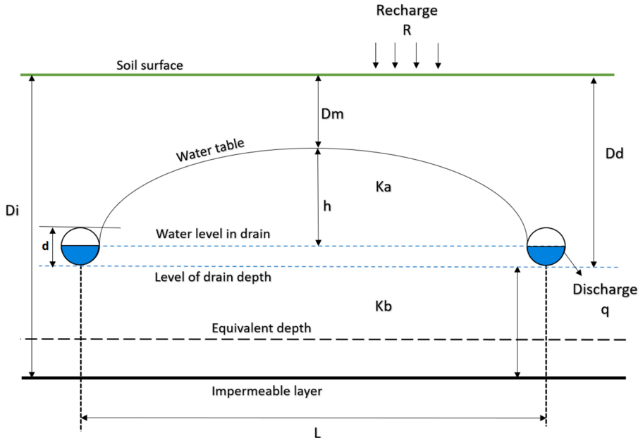
Fig. 2. Schematic of subsurface drainage system indicating input parameters for EnDrain and Eq. 4. ( D_i ) depth from the surface to impermeable layer, ( D_d ) depth of drain from surface, ( D_m ) water-table depth from surface, ( h ) height of water-table above water level in drain, ( K_a ) saturated hydraulic conductivity above the drain, ( K_b ) saturated hydraulic conductivity below the drain, ( d ) drain diameter and ( L ) is the spacing between drains.
