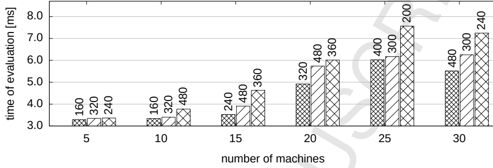
Figure 6: Best configurations (number of threads per block above each bar) of parallel evaluation on NVidia Quadro FX 570M
