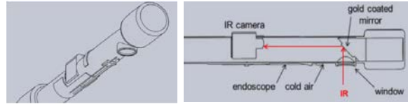
Fig. 4 Borescope design; CAD model (left) & cross-section with parts (right) [8]
