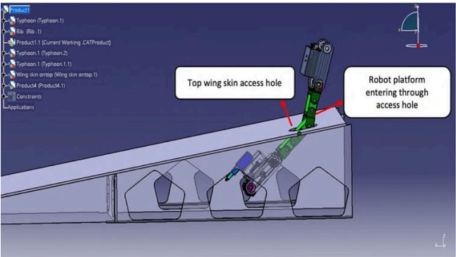
Figure 9.Robot position at entry access hole from top of wing skin
