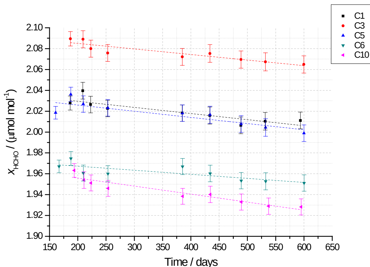
Figure 2: formaldehyde mole fraction measured in control standards during the course of the comparison versus the time since 24/08/2014 in days. Uncertainties are expressed at 95% confidence level ( k = 2 ).
