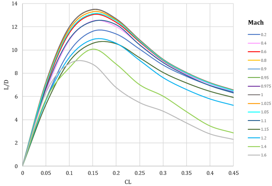
Fig. 15 High speed drag polar (lift over drag ratio vs lift coefficient) for M1.6 business jet.
