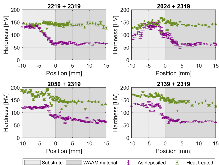
Figure 9. Vertical hardness profile before and after heat treatment for each alloy combination.
