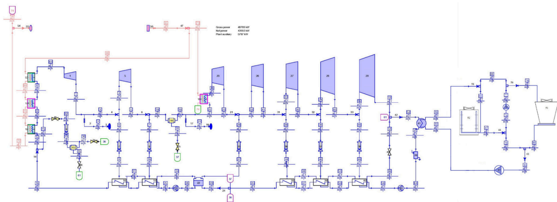
Figure 2. Thermoflex flowsheet of a 50MW e CSP plant with hybrid cooling system.
